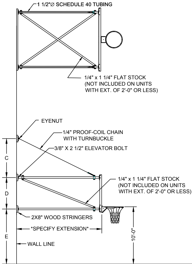
SIDE ELEVATION
